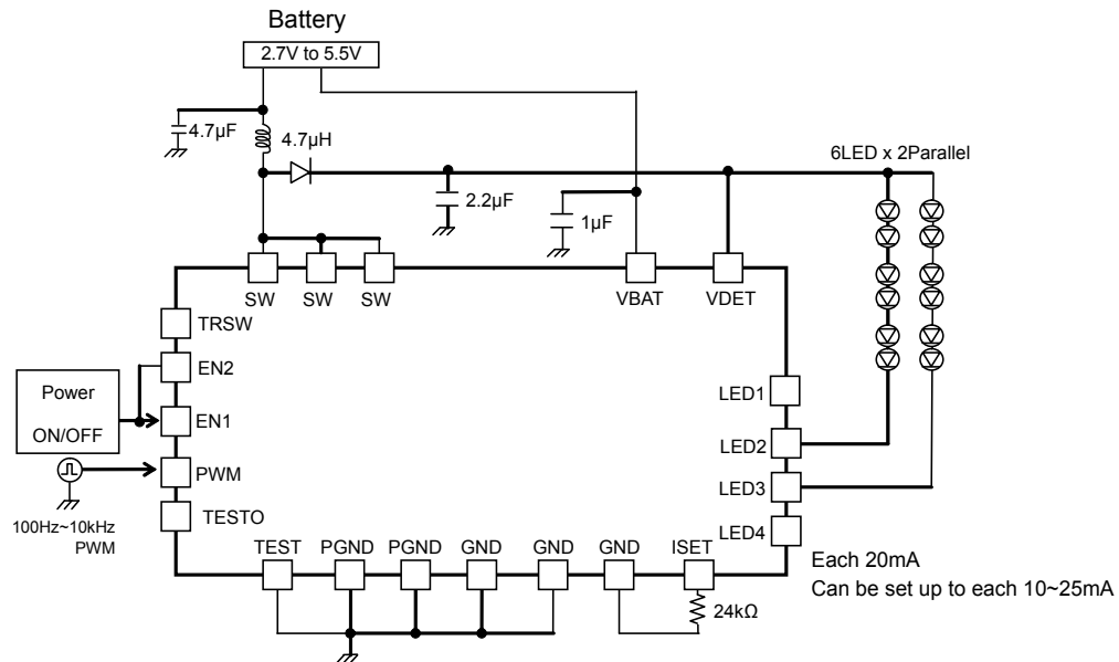
Figure 18. 6 series×2 parallel, LED current 20mA setting Current driver PWM application
