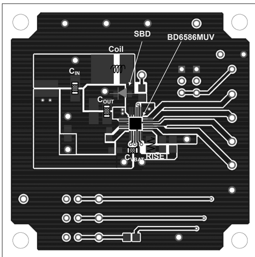
Figure 12. Frontal surface &lt;Top view&gt;
