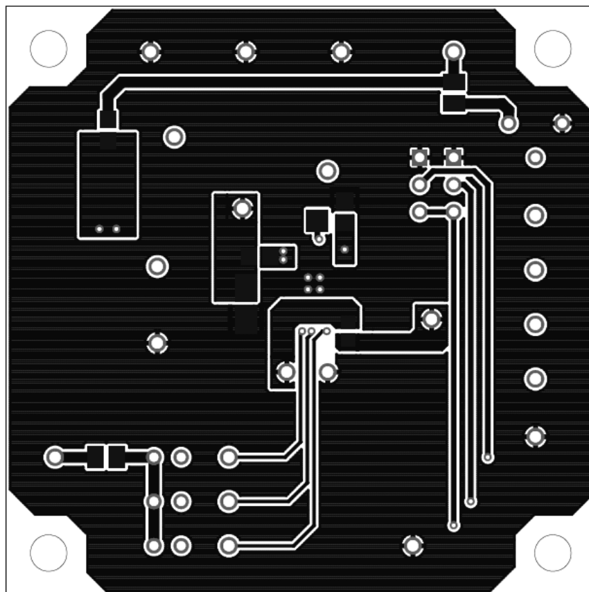
Figure 13. Rear surface &lt;Top view&gt;
